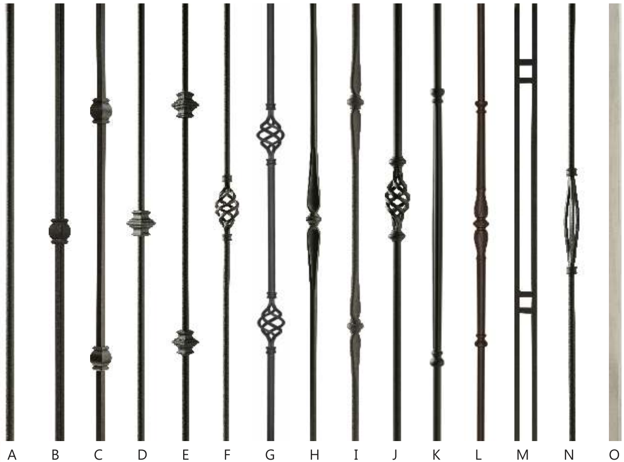
A) Plain B) Single Soft Knuckle C) Double Soft Knuckle D) Single Hard Knuckle E) Double Hard Knuckle F) Single Basket G) Double Basket H) Single Spoon Knuckle I) Double Spoon Knuckle J) Trimmed Basket K) French L) French Trimmed M) Double Trident N) Stretch Basket O) Rectangular Series
